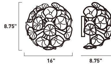
E22092-26, -28 Wall/Flush Mount
