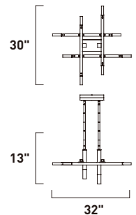
Frame diagram and overall measurements
