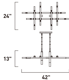
Frame diagram and overall measurements
