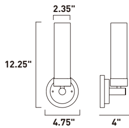
E63106-11SN Wall Mount
