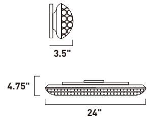
E24041-20PC Bath Vanity
