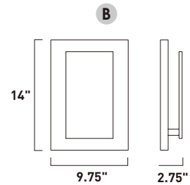
E41335-BKSA, -WT Interior/Exterior Wall Sconce
